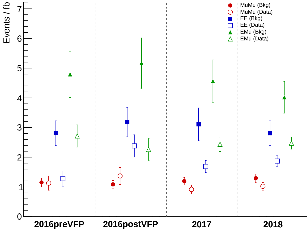
Total Background vs Data: PassCR3_MET_HighJet, HNTightV2
