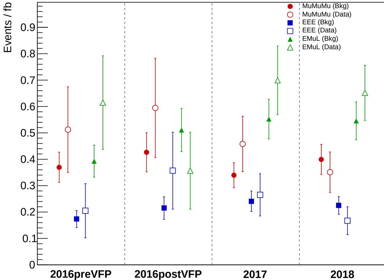
Total Background vs Data: HNL_WZVBF_ThreeLepton_CR, HNTightV2
