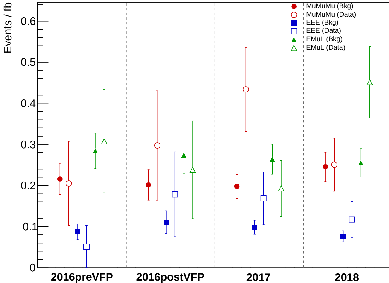
Total Background vs Data: HNL_WZ_SR1_ThreeLepton_CR, HNL_ULIDv2
