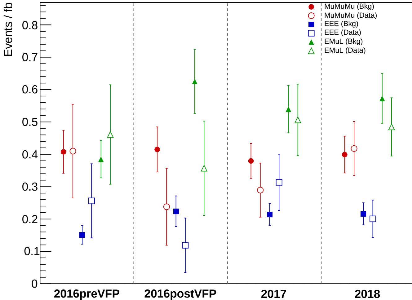
Total Background vs Data: HNL_WZ_SR1_ThreeLepton_CR, HNTightV2
