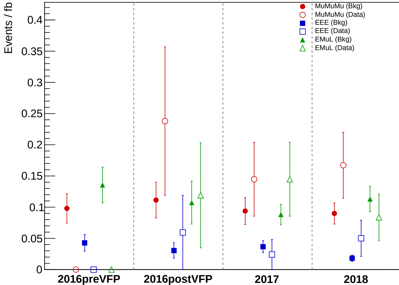
Total Background vs Data: HNL_WZ_SR1_ThreeLepton_CR, POGTight
