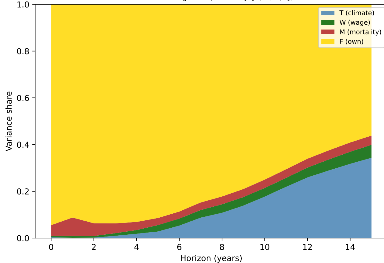
C. FEVD of log CBR (Cholesky [T,W,M,F])
