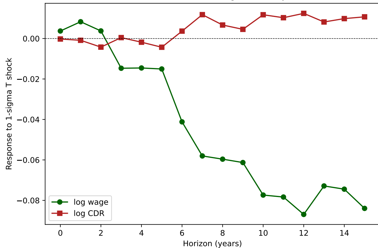
D. Mediation share via ordering swap
