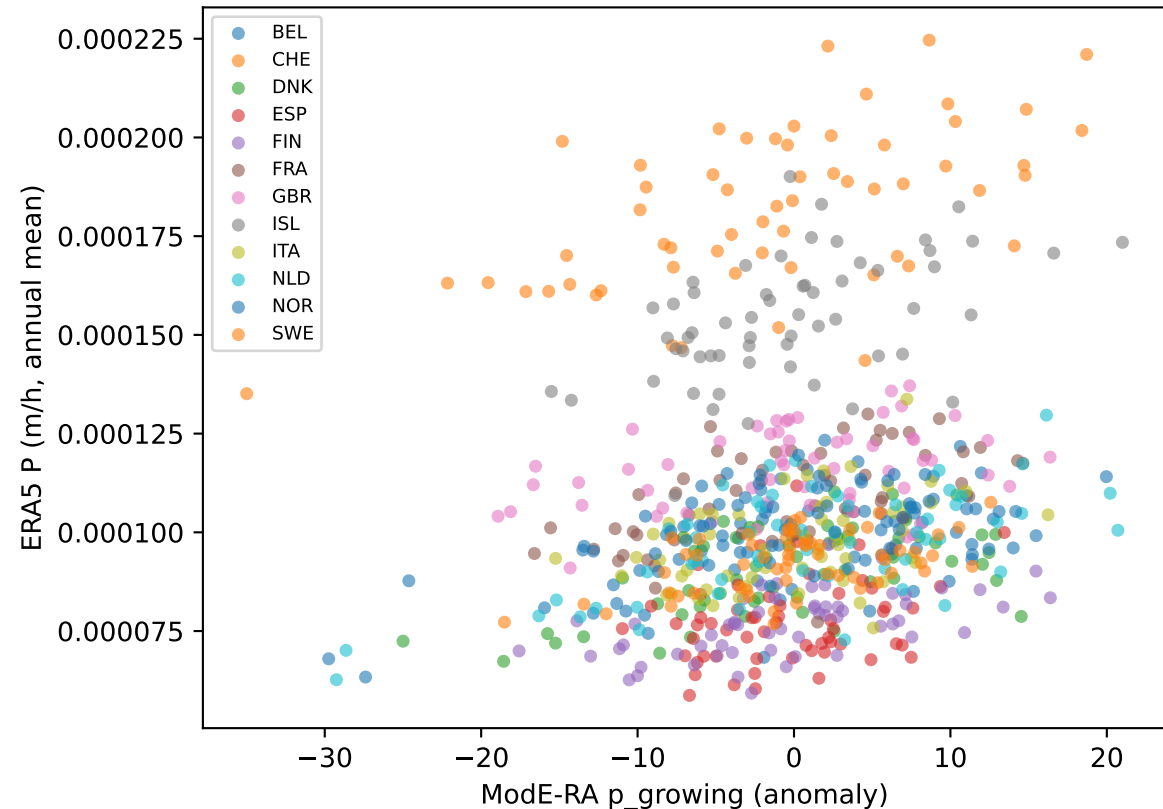
B. Precipitation (1950-2008)
