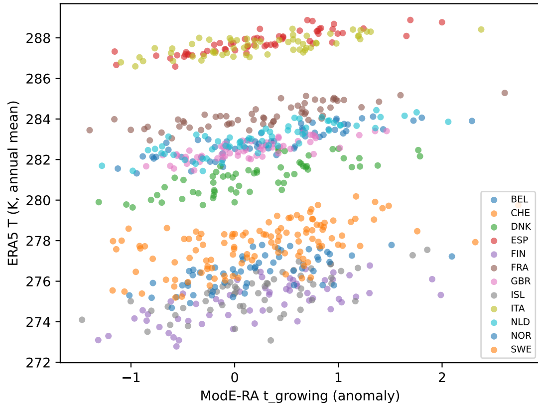
A. Temperature (1950-2008)
