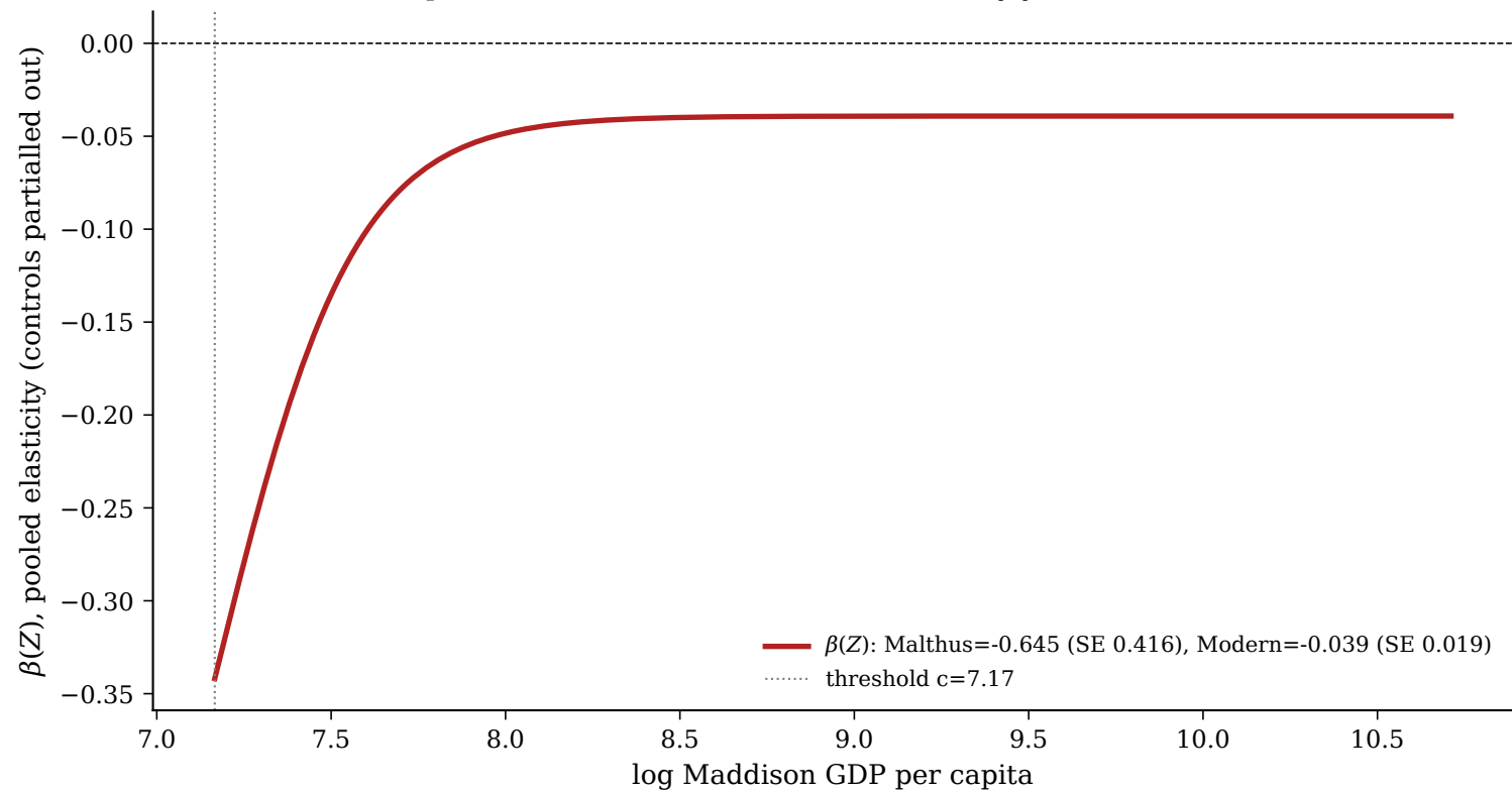
Phase 2 pooled smooth-transition, N=1413 country-years across 7 countries
