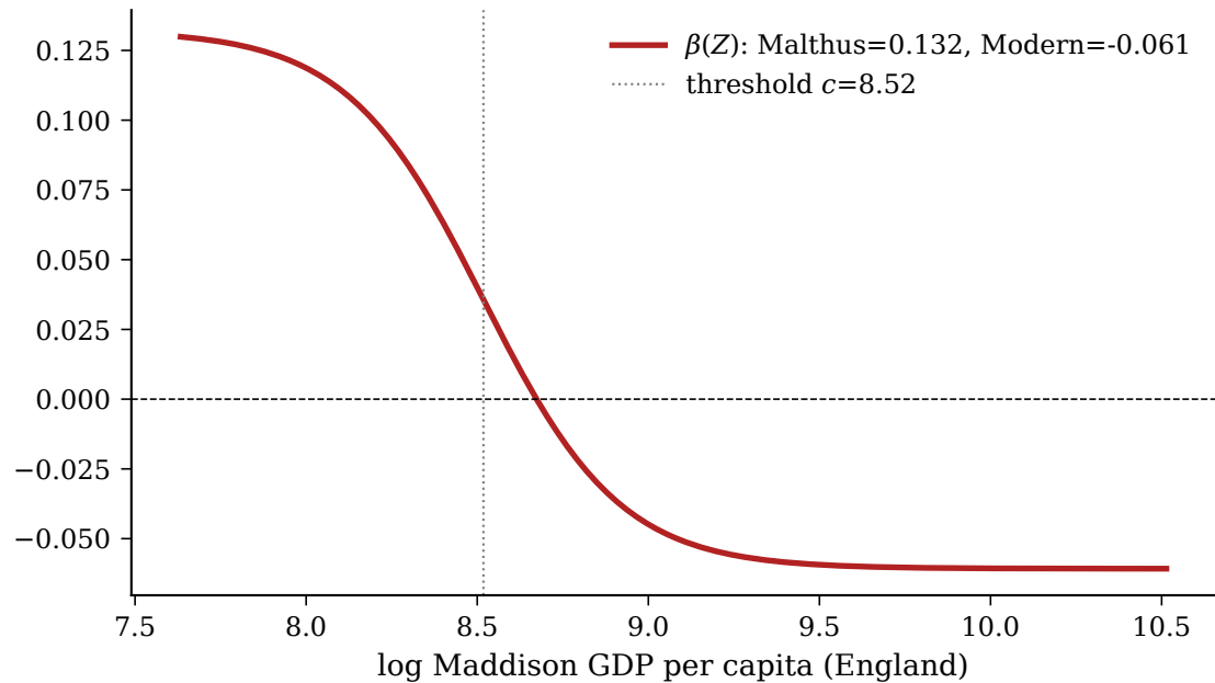
Smooth-transition \beta(Z)
