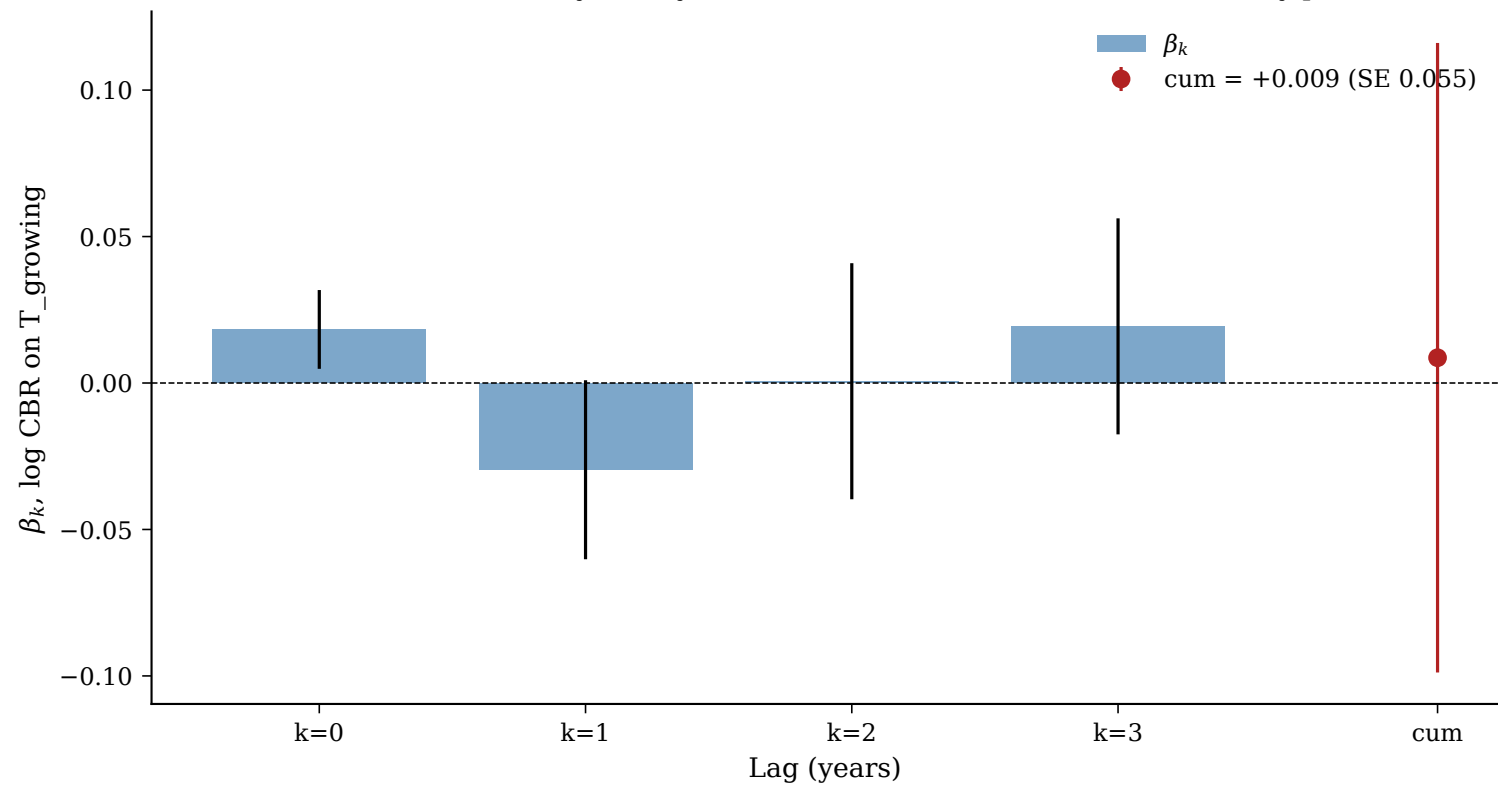
Pooled DL IRF (country FE + year FE + 9 controls + cluster SE), 4-country panel
