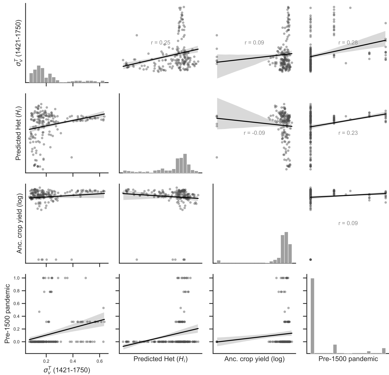
Figure 1: Substrate covariance — four pre-industrial deep determinants
