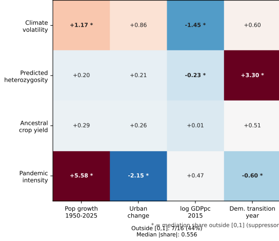
Figure 5 — Mediation-share robustness: pathway-source comparison 4 substrates × 4 modern outcomes Climate-only-clustered pathways (Exercise 2) Mediator: K = 5 on climate primitives
