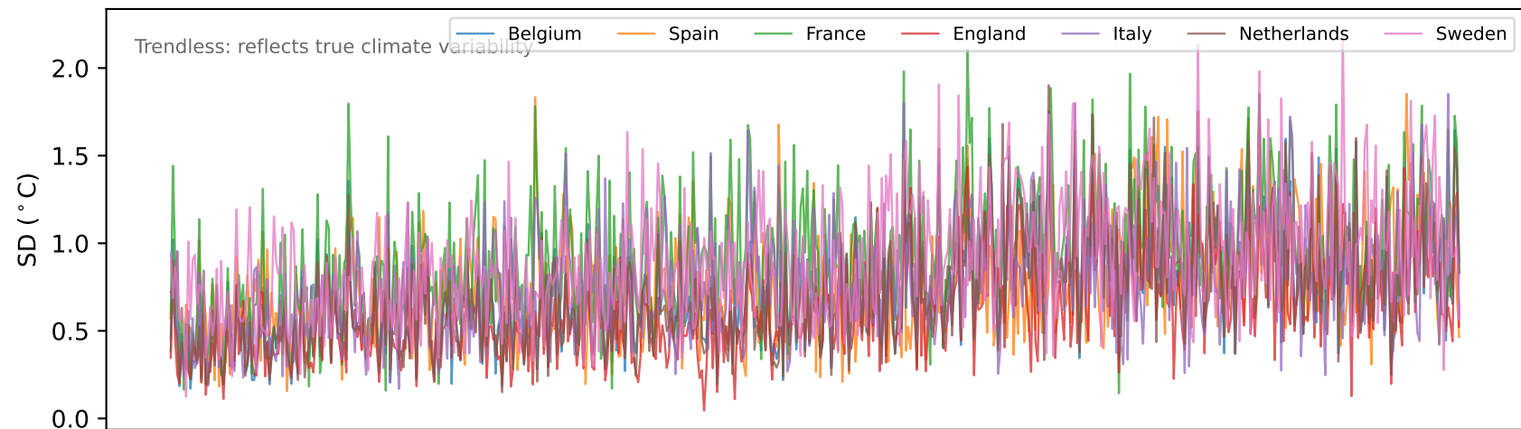
Headline: within-growing-season realized SD of monthly temperature anomaly
