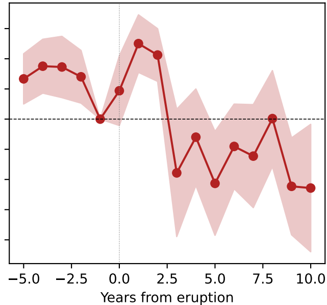
Pinatubo (1991) — with controls
