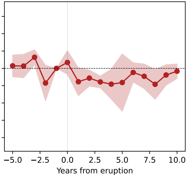
Tambora (1815) — with controls
