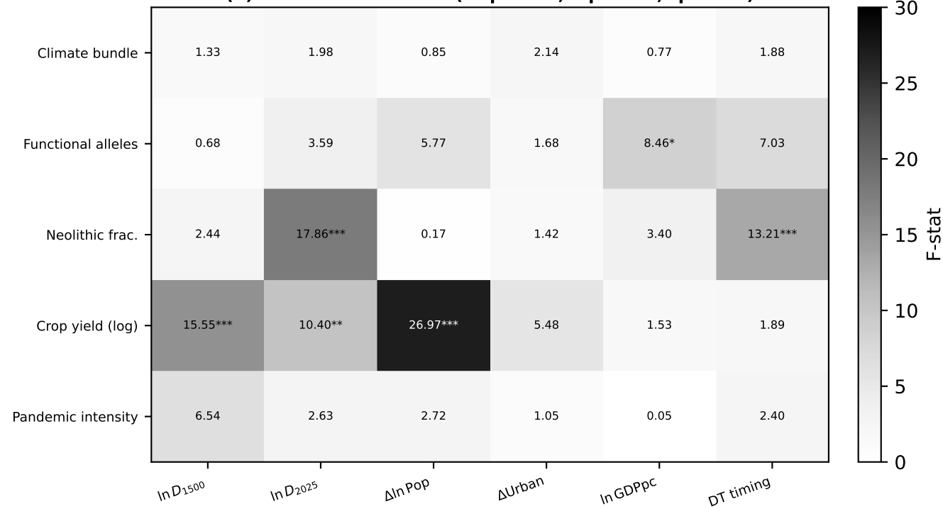
(f) Outcome heterogeneity: DT timing, full vs early-transition
