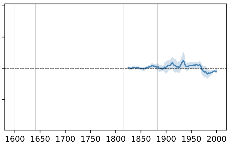
Phase 5 rolling-window IRF -- 7 countries (gap-filled England via HMD)
