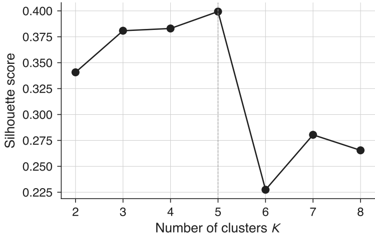
(a) Silhouette score by K
