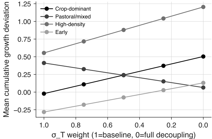
(b) CF3: climate decoupling
