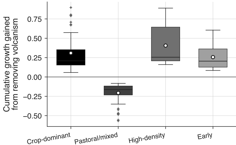
(a) CF2: no 1500–1900 volcanism
