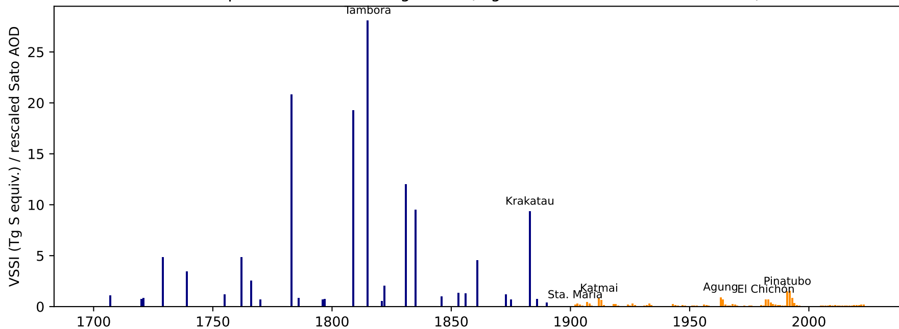
Fig 13v2 — Extended volcanic IV reaching Pinatubo 1991
