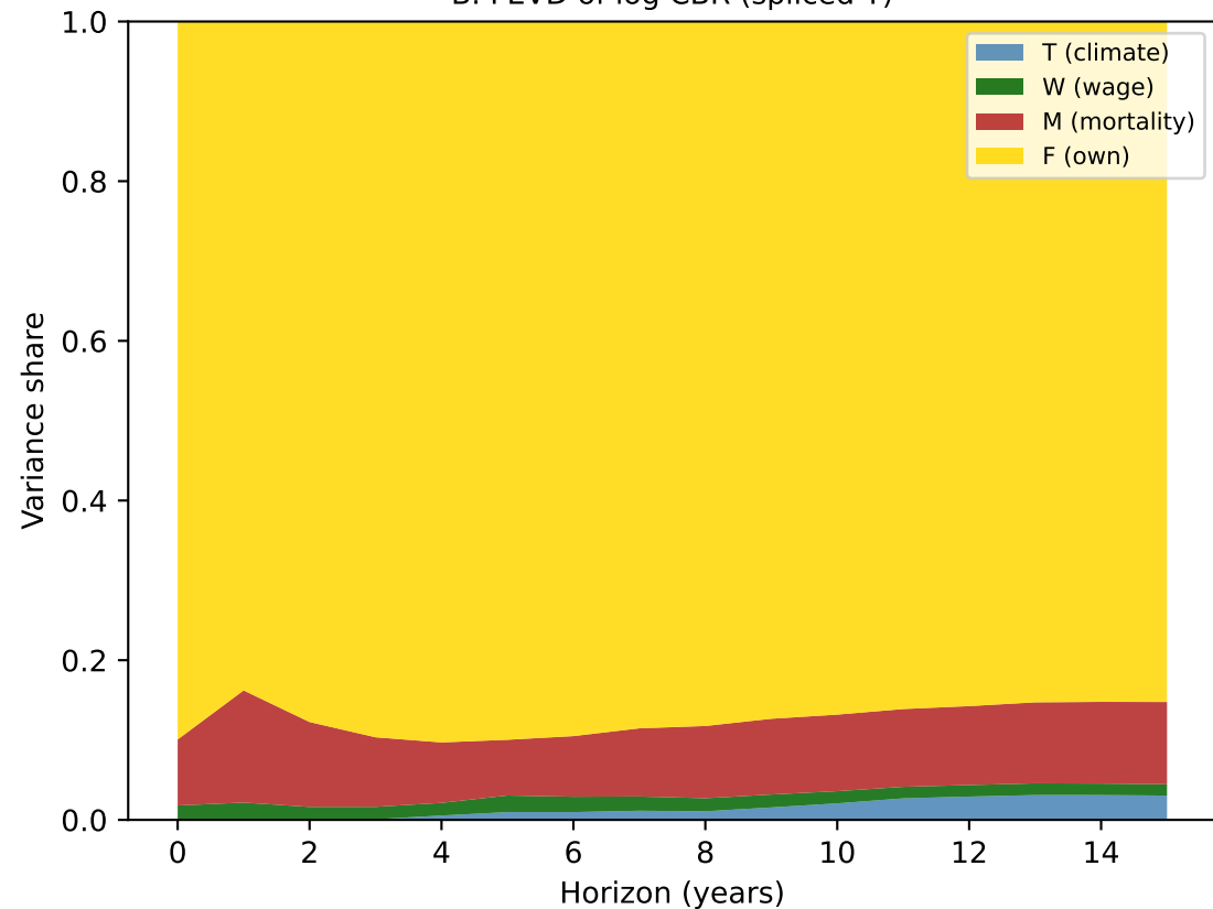
B. FEVD of log CBR (spliced T)
