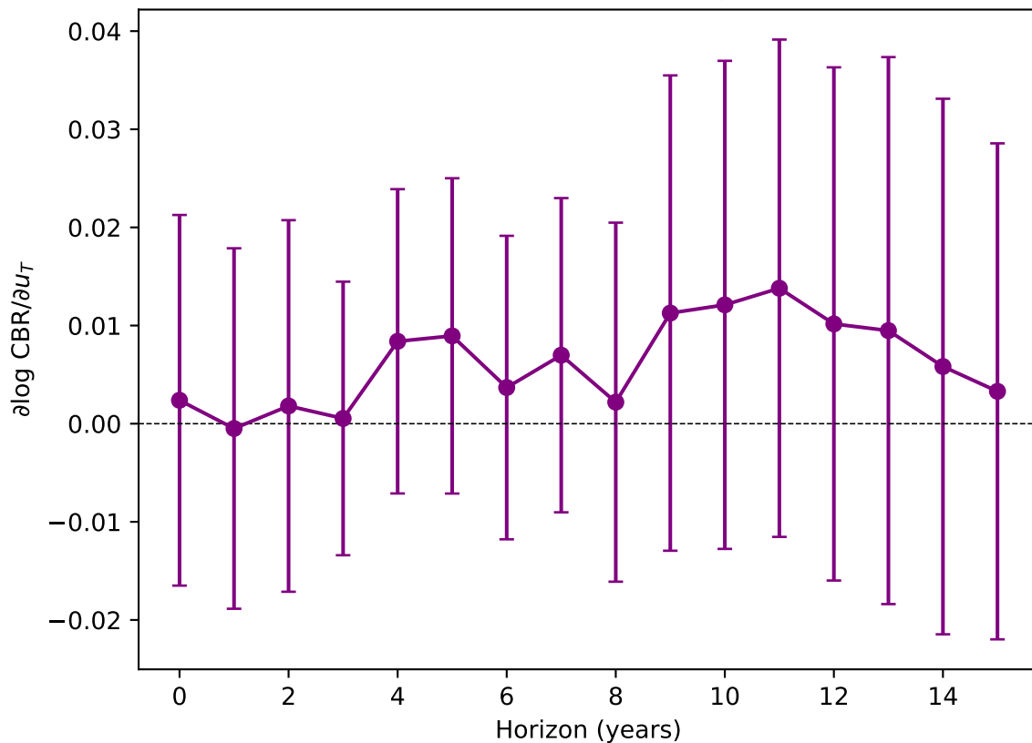
A. IRF F < -T (ModE-RA+ERA5 spliced T)
