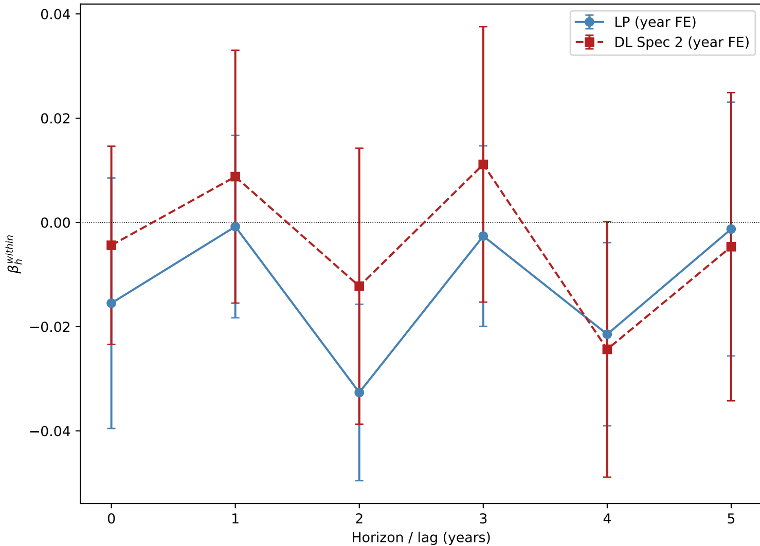
Fig 19 — France dept system LP IRF (within-country, year-FE identified)
