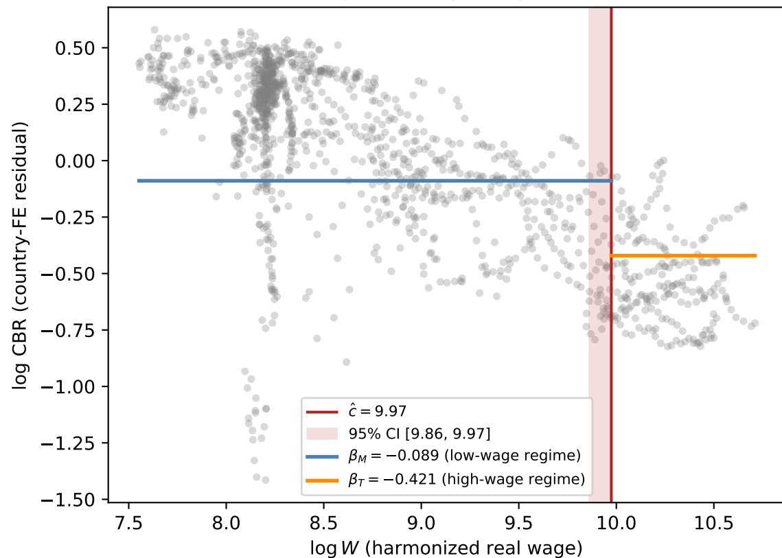
A. Threshold regression (sup-Wald p=0.012 , N=1314 )
