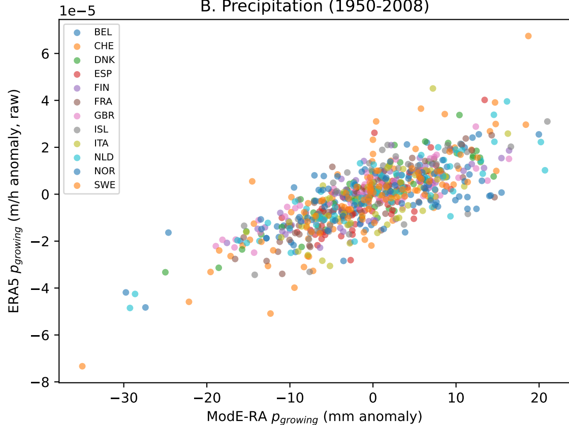
B. Precipitation (1950-2008)
