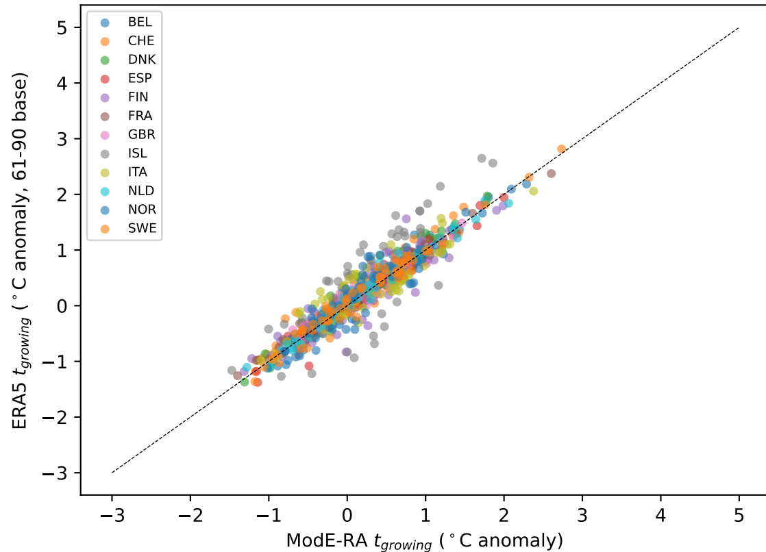
A. Temperature (1950-2008)
