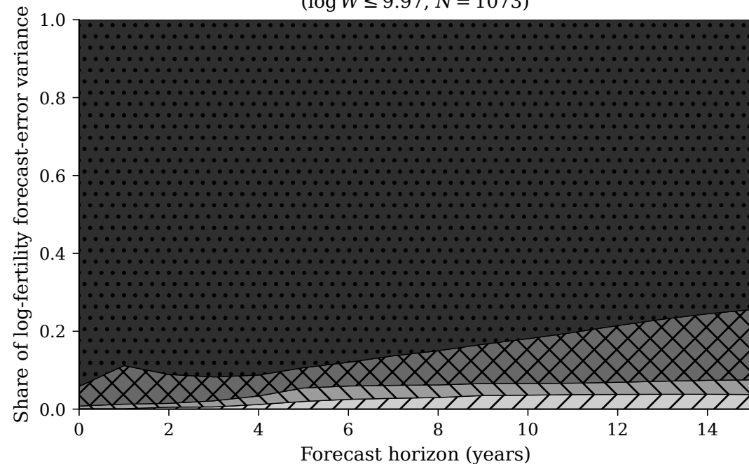
Malthusian regime ( \log W \leq 9.97 , N = 1073 )
