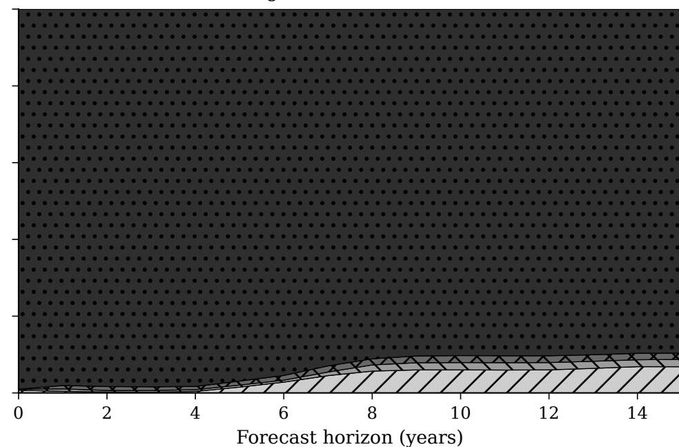
Modern regime ( \log W > 9.97 , N = 367 )
