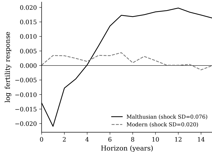
(A) Response to a 1-s.d. mortality shock, by regime
