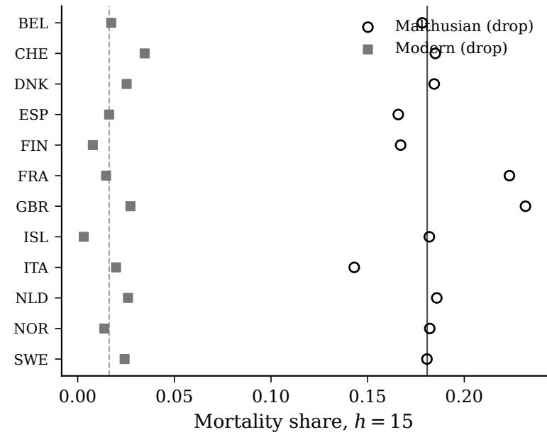
(C) Leave-one-country-out (lines = headline)
