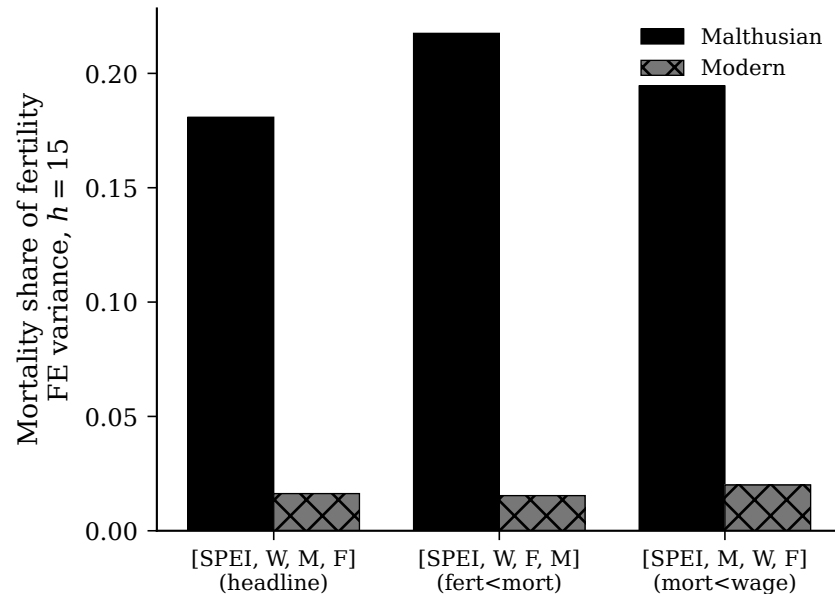
(B) Cholesky ordering swaps
