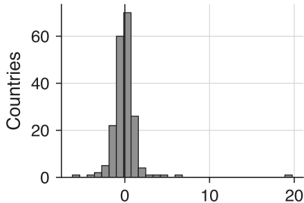
(a) Mean bias median |b| = 0.61^{\circ}\text{C}
