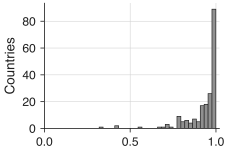
(b) Monthly correlation median = 0.971
