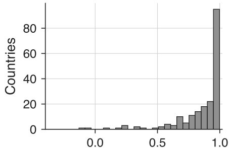
(c) Year-to-year skill median = 0.938
