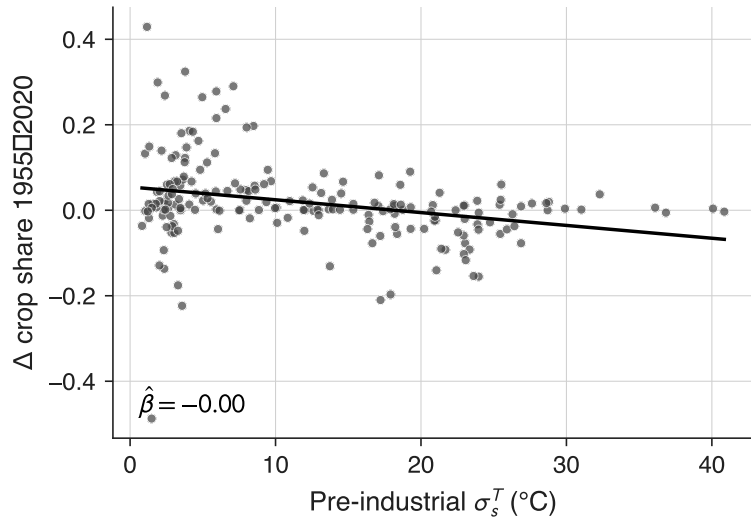
(b) Intra-annual range \rightarrow \Delta crop share
