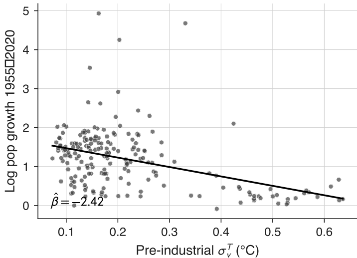
(a) Inter-annual volatility \rightarrow pop growth
