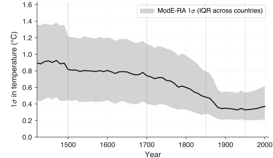
(c) Temperature uncertainty by decade
