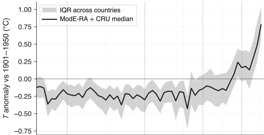
(c) Temperature uncertainty by decade
