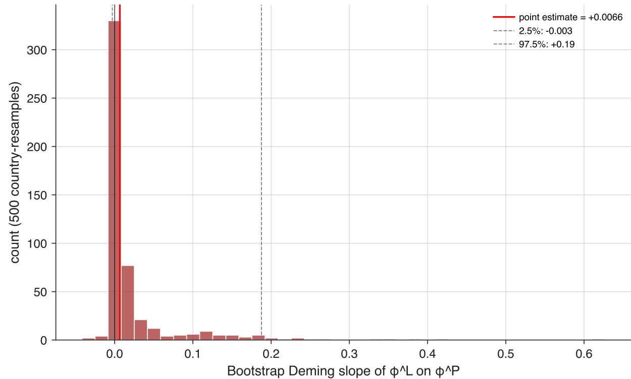
(b) Bootstrap distribution, P(\text{slope} < 0) = 0.09
