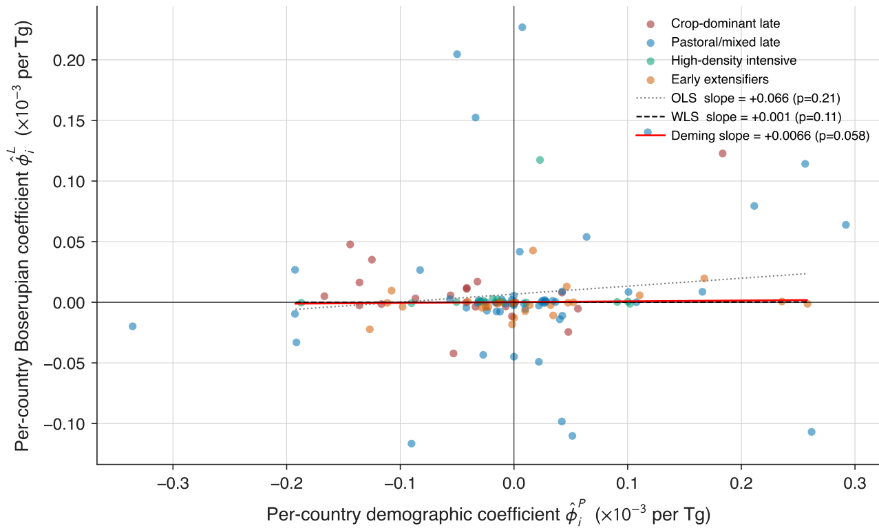
(a) Country-level ( \phi^P , \phi^L ) scatter, post-1700
