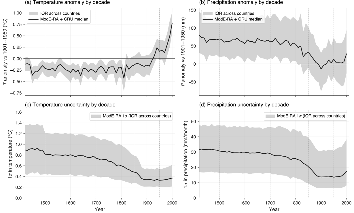
Figure 6: The ModE-RA climate panel, 1421–2008: levels (top row) and uncertainty (bottom row). (a) Temperature anomaly versus the 1901–1950 reference; (b) precipitation anomaly. (c–d) Country-month 1\sigma uncertainty by decade: the grey band is ModE-RA’s published ensemble standard deviation, the working uncertainty propagated into the regressions. Absolute levels are anchored to the CRU 1901–1950 climatology.
