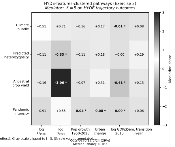
Figure 7: Pathway-cluster-source robustness: mediation matrices under climate-only-clustered pathways (left, the baseline) and HYDE-features-clustered pathways (right). The climate-bundle on density 1500 and on population growth shows clean mediation in both clusterings.
