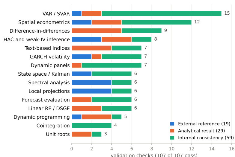
Figure 1: The validation gallery of puremacro 3.3.0: 107 checks in 15 subsystems, by kind of reference; all pass. External reference : stored outputs of statsmodels, arch, linearmodels or esda, SciPy computed at run time, or a published table. Analytical result : a closed form, or an effect planted in simulated data. Internal consistency : agreement between alternative algorithms, identities that correct output must satisfy, or recovery of parameters from simulated data. Regenerate with python paper/make_scorecard_fig.py.
