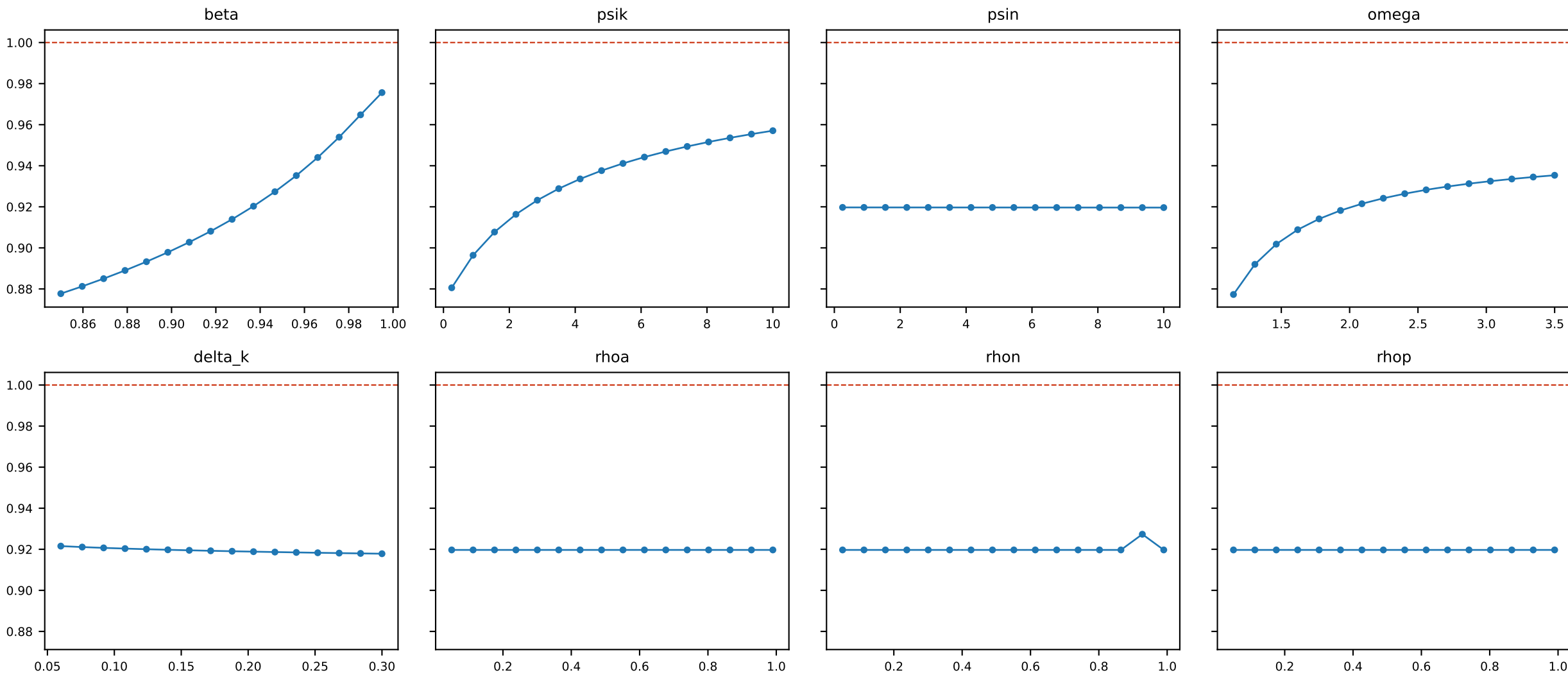
Boundary-root modulus, 1-D sweeps around the healthy (Bayesian .mod) calibration, exact SS
