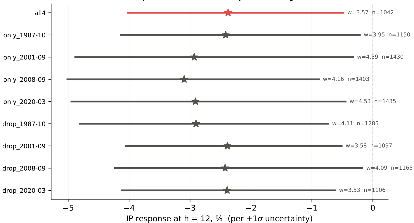
Narrative event-set sweep: 68% band at h = 12 by event configuration (baseline dataset)
