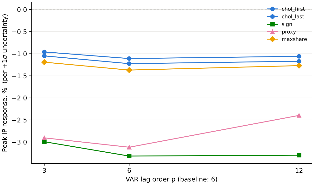
Lag-order sweep, baseline dataset
