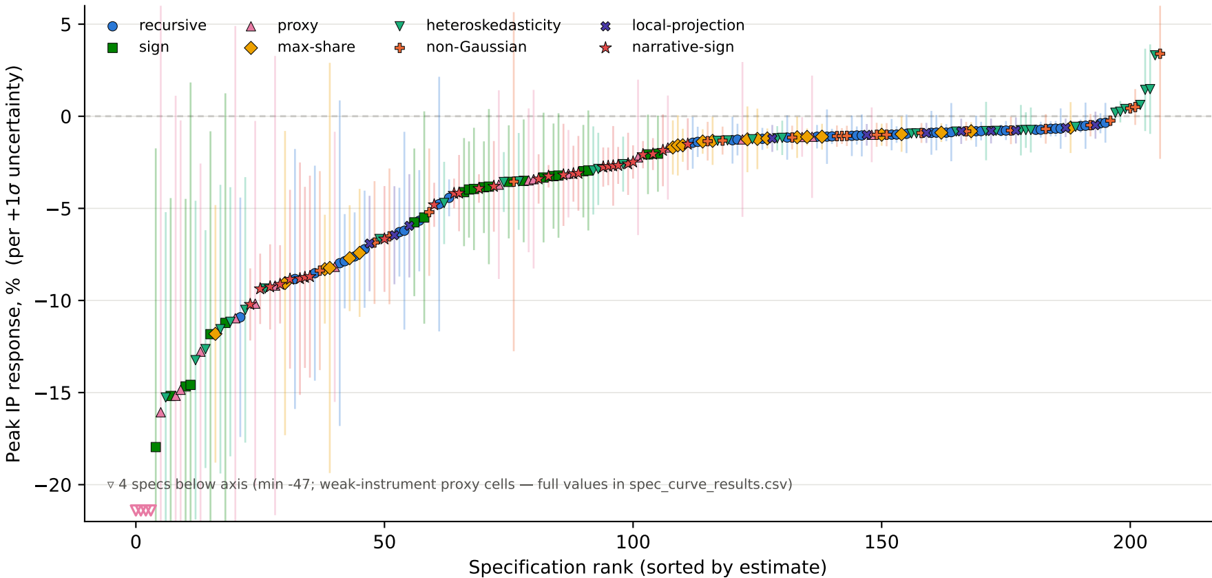
Peak activity response to an uncertainty shock across 207 specifications
