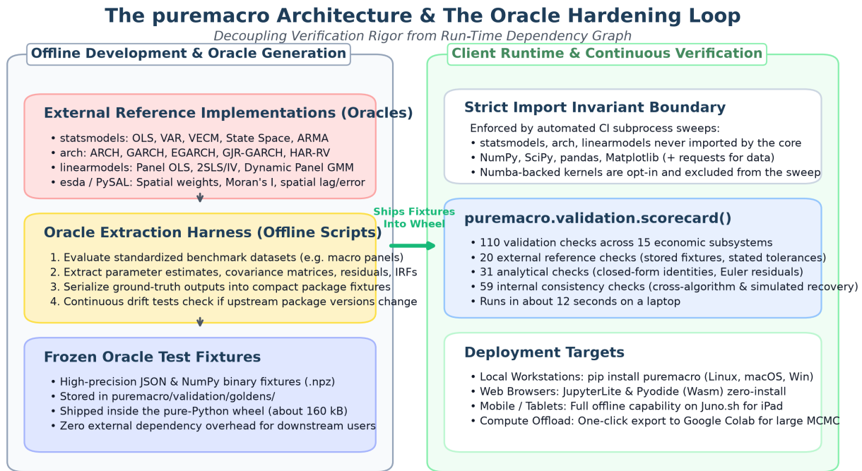
Figure 2: Software Architecture and the Oracle Hardening Loop in puremacro . The schematic illustrates the decoupling between the offline verification environment and the client runtime. In the offline factory (left), established external packages ( statsmodels , arch , linearmodels , and esda ) compute oracle estimates on standardized macroeconomic datasets, serializing reference fixtures into compact package files. In the client environment (right), a strict import boundary forbids oracle libraries from entering the runtime. The self-contained gallery puremacro.validation.scorecard() illustrates the validation workflow; it does not certify all deployment targets. Counts are those of release 4.5.0; tolerances are case-specific, and the gallery’s browser run time has not been measured.
