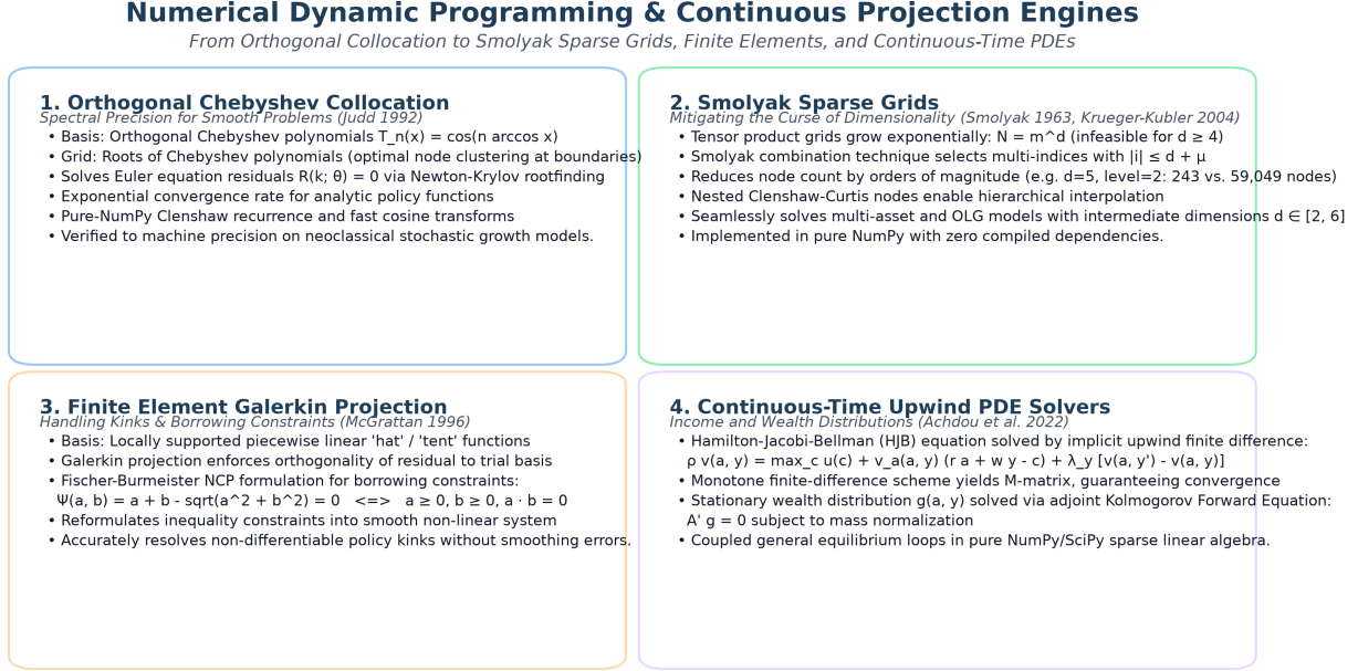
Figure 5: Continuous State-Space Projection and Numerical Dynamic Programming Engines in puremacro . The four quadrants contrast complementary numerical approaches: (1) orthogonal Chebyshev polynomial collocation on smooth problems (Judd, 1992); (2) Smolyak multidimensional sparse grid interpolation mitigating the curse of dimensionality (Smolyak, 1963; Krueger and Kubler, 2004); (3) finite element Galerkin projection with Fischer-Burmeister NCP complementarity for non-differentiable borrowing kinks (McGrattan, 1996); and (4) continuous-time implicit upwind PDE solvers for stationary wealth distributions (Achdou et al., 2022).
