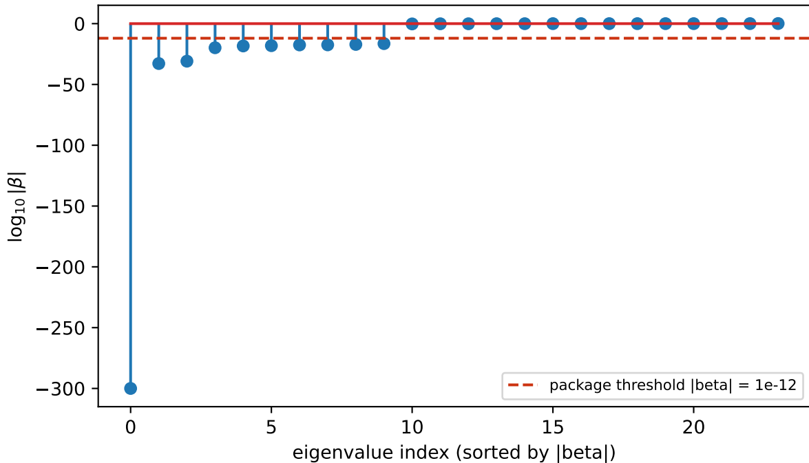
QZ |\beta| clusters: finite vs infinite eigenvalues
