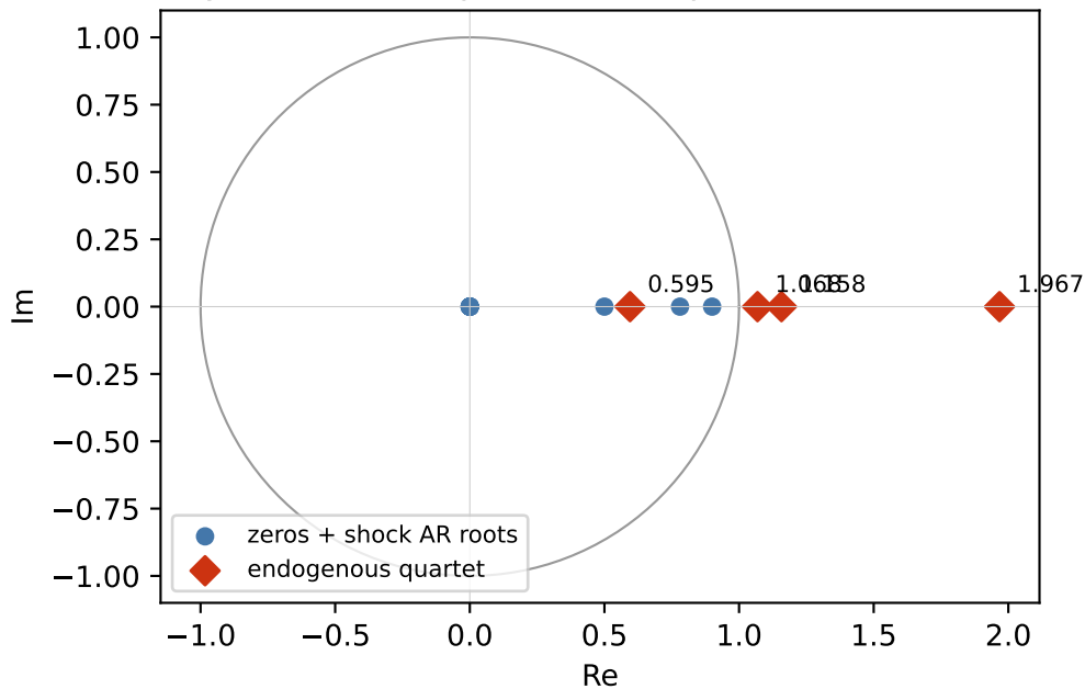
Fertility DSGE: finite pencil roots (port default calibration)
