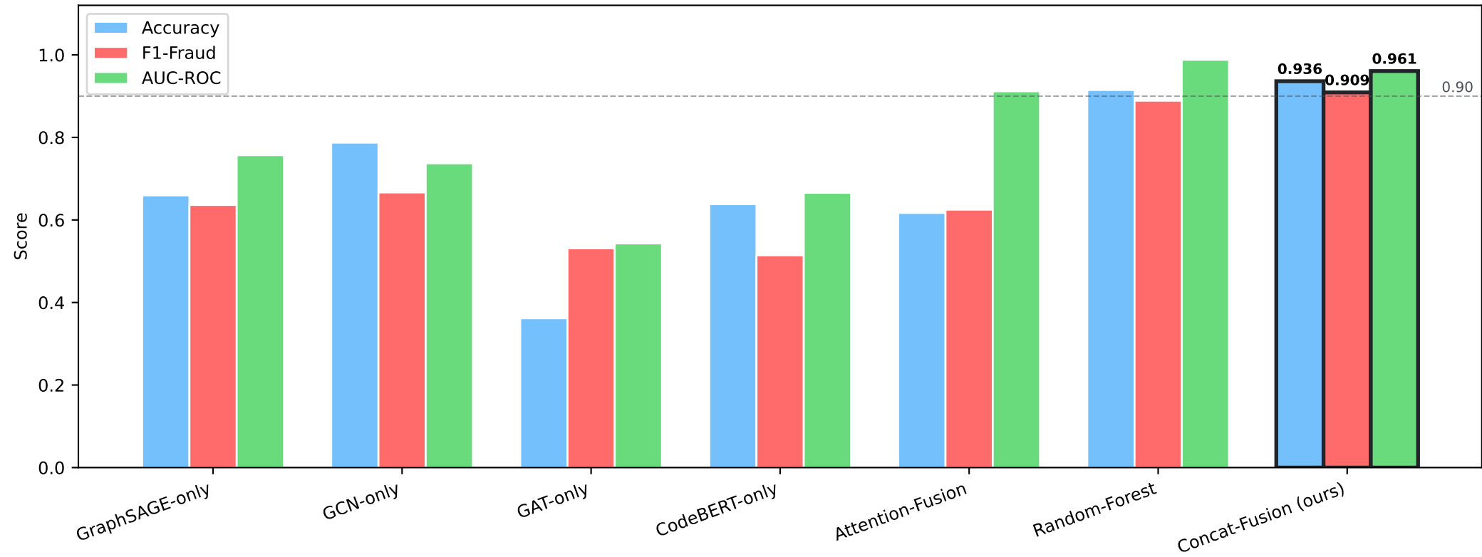
Ablation Study: Model Comparison on Test Set
