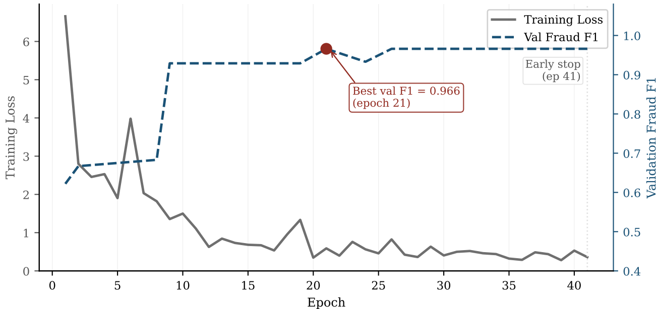
Training Loss and Validation Fraud F1
