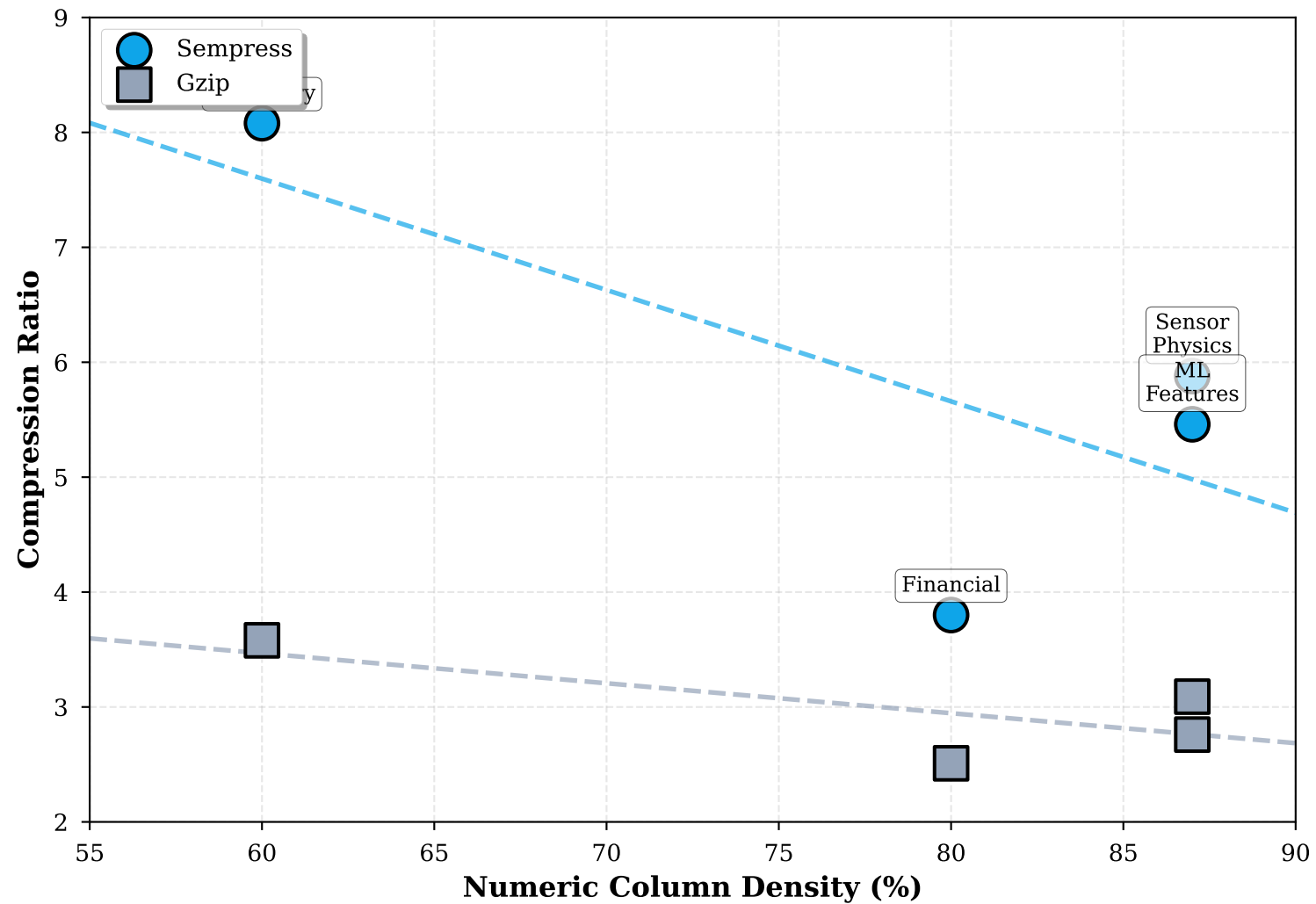
Compression Ratio vs. Numeric Density
