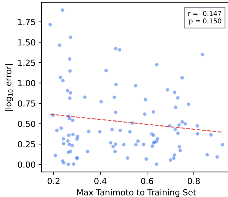
B. Error vs Chemical Similarity
