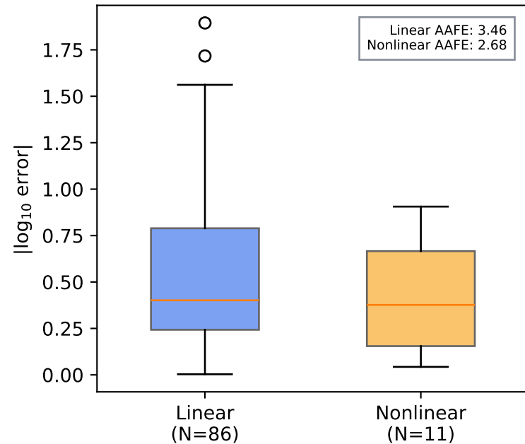
A. Error by PK Linearity
