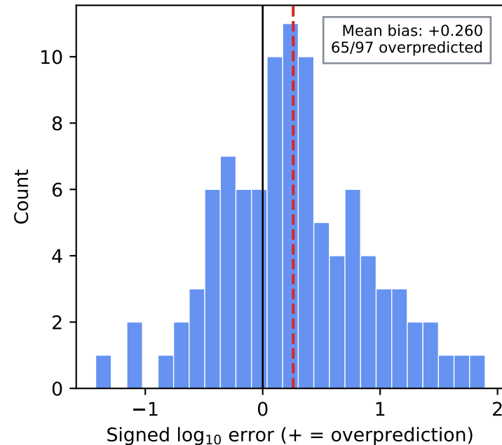
C. Prediction Bias Distribution
