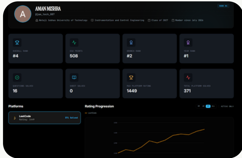
Profile & Insights
