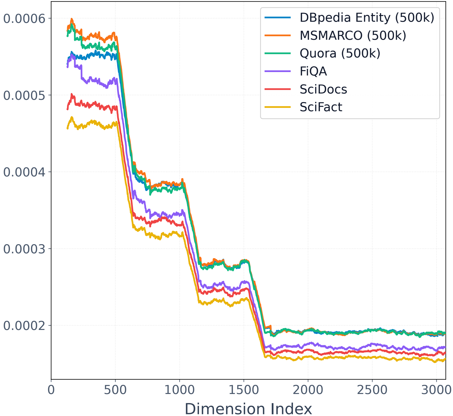
Rolling Mean Variance (Window=128)
