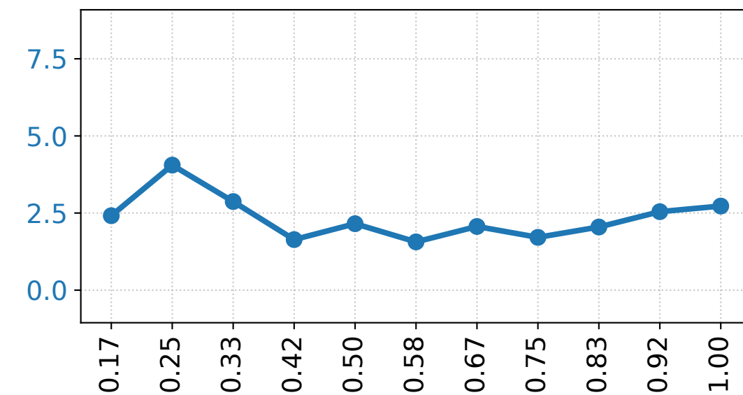
SciFact
