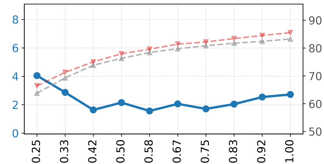
SciFact
