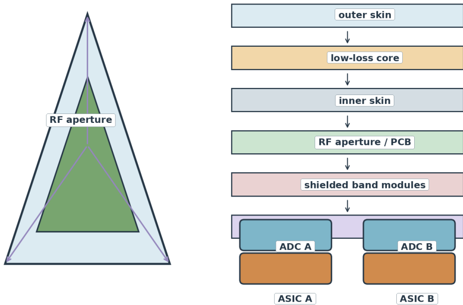
Figure 5.1: Triangular RF face module and exploded stack: the left triangle represents aperture, calibration and structural paths; the right coloured plates represent successive RF, dielectric, shielding, processing, thermal and service layers.
