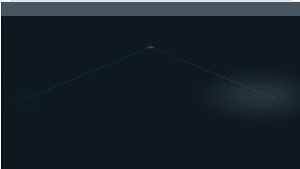
Figure 7.1: Two-node aircraft scenario: the two enlarged radomes define the nominal 100 km baseline, the aircraft is above and offset from it, and the blue/red paths and cones represent independent received signals and angular observations used for power, AOA, TDOA and Doppler consistency.
