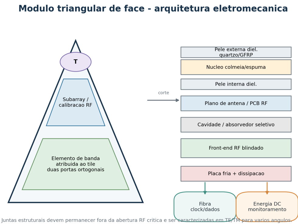
Figure 5.1: Triangular RF face module / Módulo triangular de face RF.
