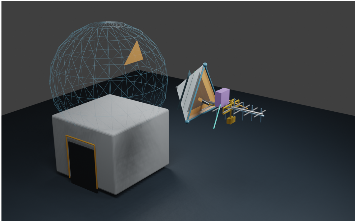
Figure 3.6: Blender Eevee render of the radome and exploded face. The external VHF Yagi uses a support/boom axis continuing from the internal apex; its parasitic elements are transverse to that axis.
