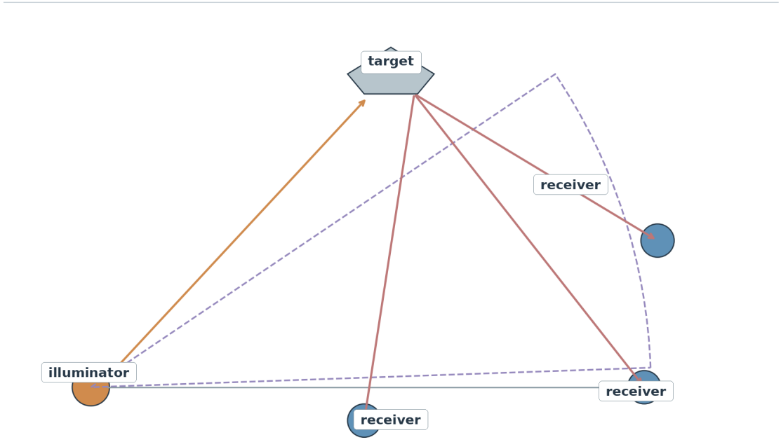
Figure 6.2: Bistatic/multistatic geometry: the orange point is the illuminator, the upper polygon is the target, blue points are receivers, orange and red paths are illumination and target-to-receiver propagation, and the dashed arc represents an equal-delay locus.
